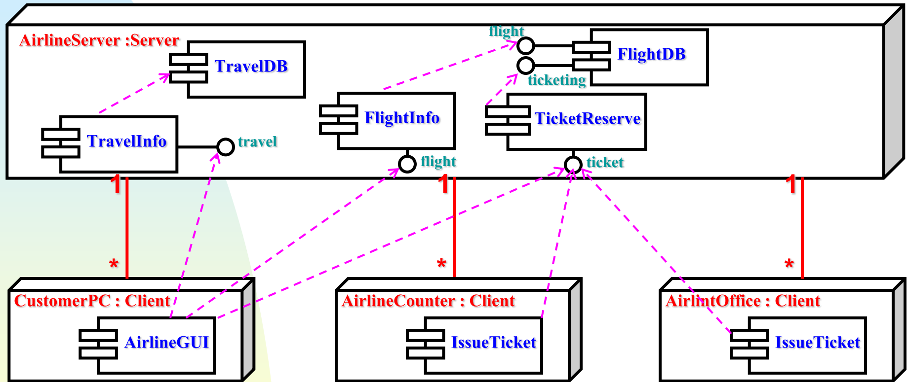
Deployment Diagram : Airline Reservation System
